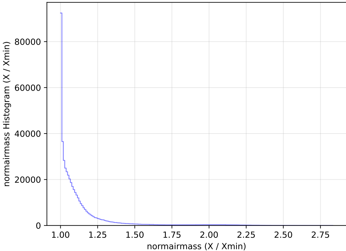
noroll_mjdp60_v3.4_10yrs All sky r band: normairmass Histogram
