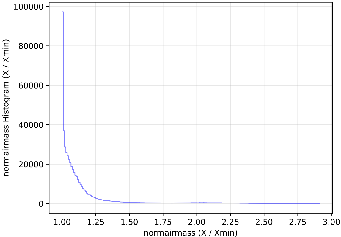
noroll_mjdp60_v3.4_10yrs All sky i band: normairmass Histogram
