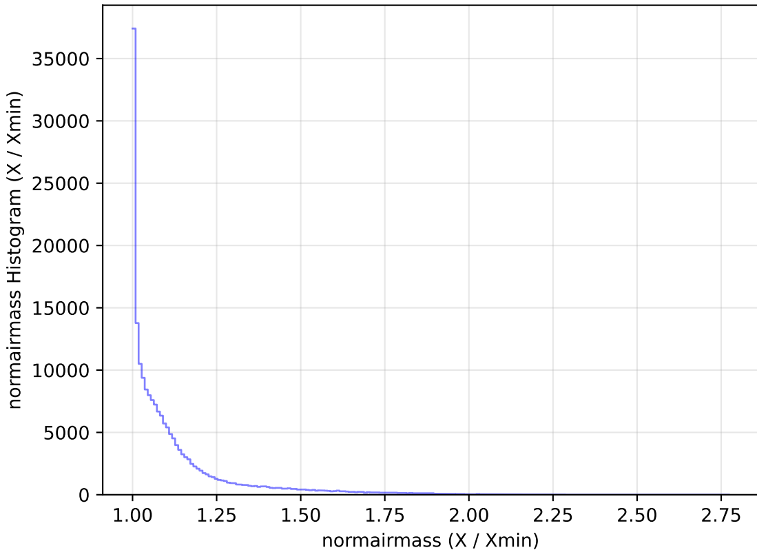
noroll_mjdp60_v3.4_10yrs All sky g band: normairmass Histogram
