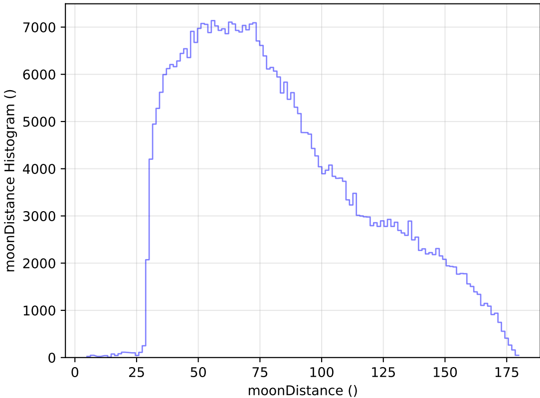
noroll_mjdp60_v3.4_10yrs WFD z band: moonDistance Histogram
