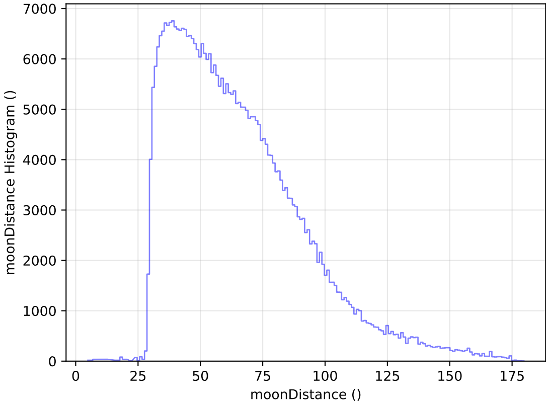
noroll_mjdp60_v3.4_10yrs WFD y band: moonDistance Histogram
