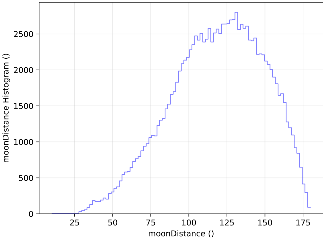
noroll_mjdp60_v3.4_10yrs WFD u band: moonDistance Histogram
