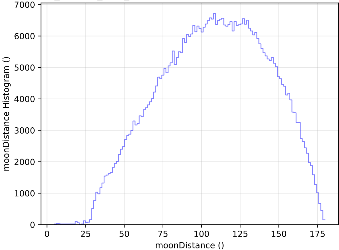
noroll_mjdp60_v3.4_10yrs WFD r band: moonDistance Histogram
