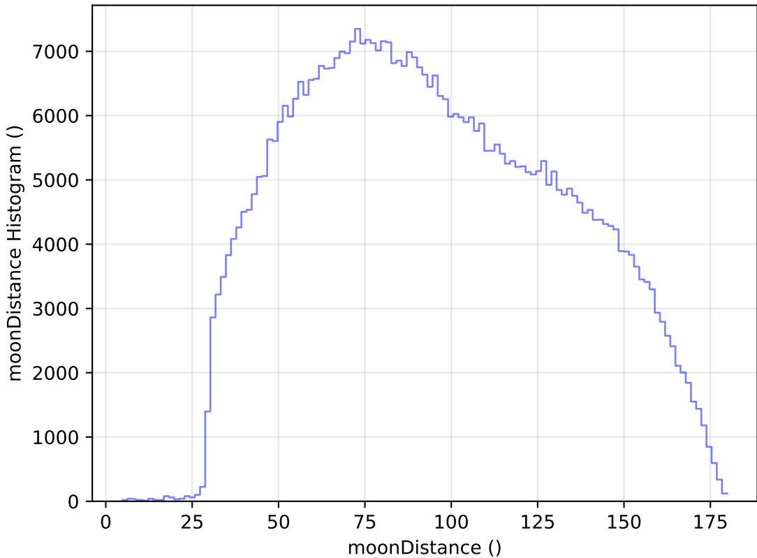
noroll_mjdp60_v3.4_10yrs WFD i band: moonDistance Histogram
