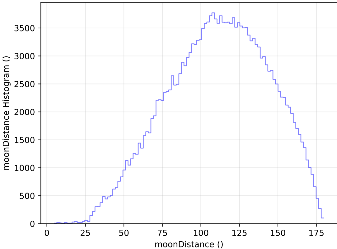
noroll_mjdp60_v3.4_10yrs WFD g band: moonDistance Histogram
