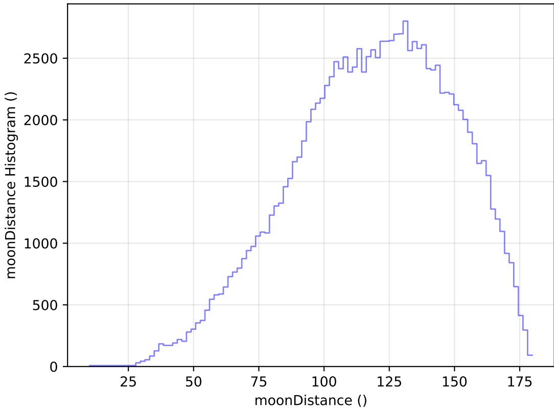
noroll_mjdp60_v3.4_10yrs All sky u band: moonDistance Histogram
