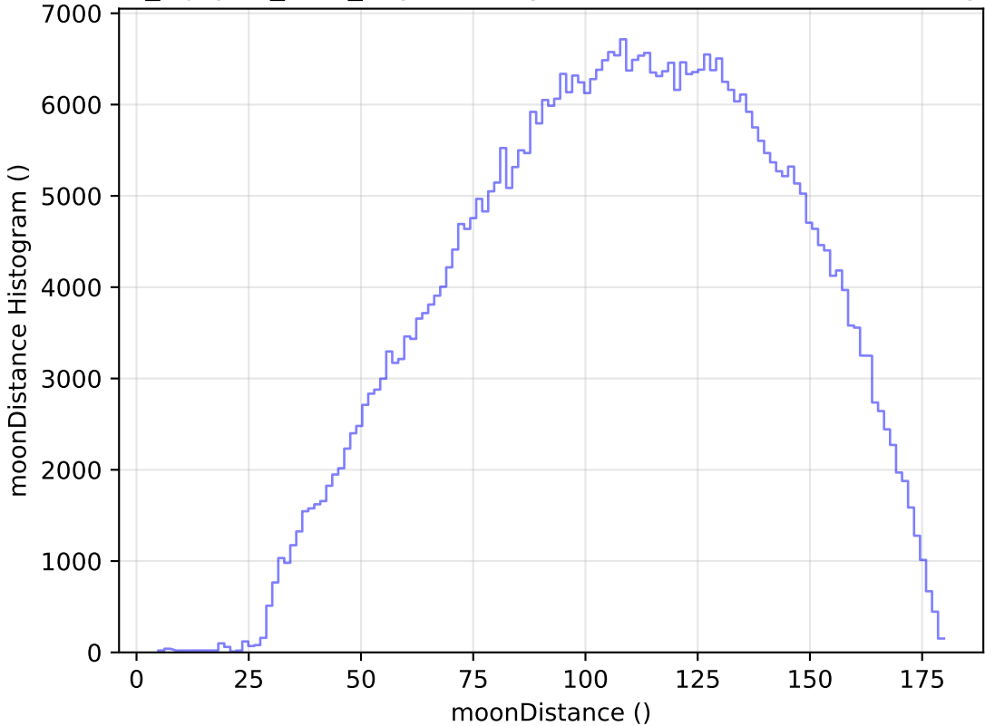
noroll_mjdp60_v3.4_10yrs All sky r band: moonDistance Histogram
