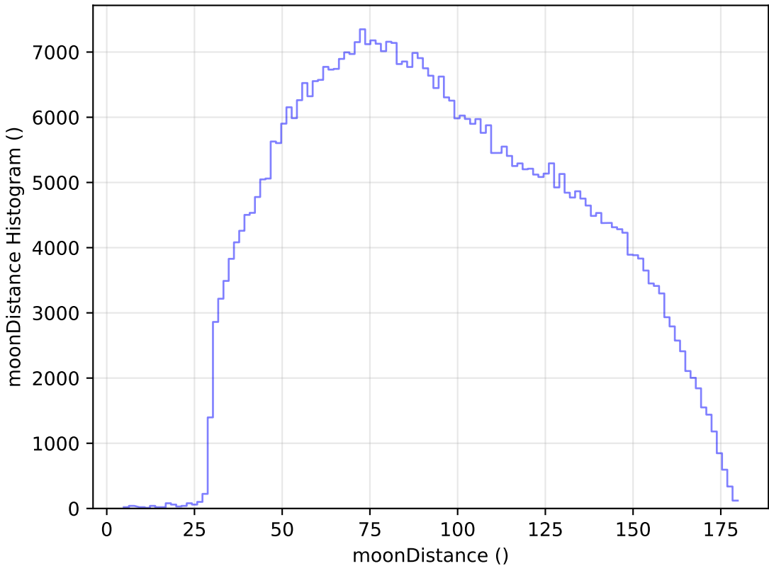
noroll_mjdp60_v3.4_10yrs All sky i band: moonDistance Histogram
