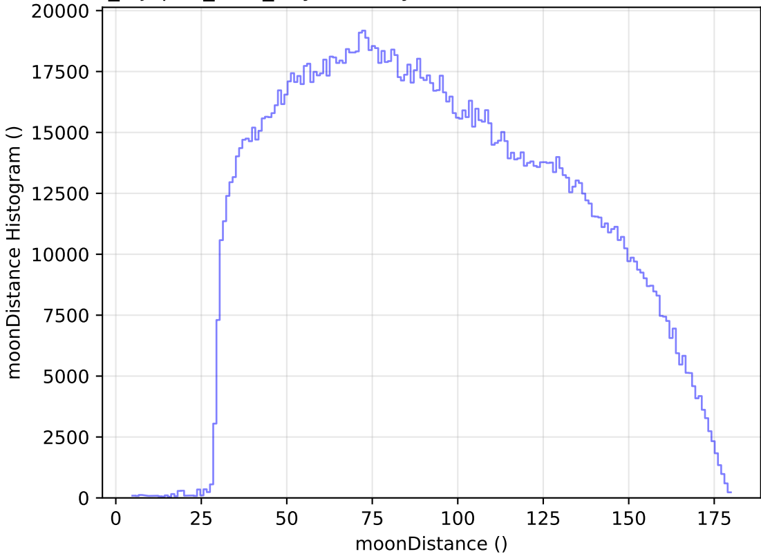
noroll_mjdp60_v3.4_10yrs All sky all bands: moonDistance Histogram
