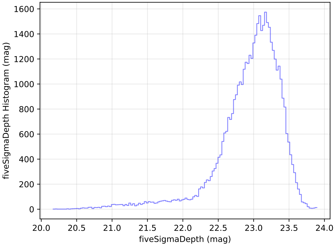
noroll_mjdp60_v3.4_10yrs Yr 1 z band: fiveSigmaDepth Histogram
