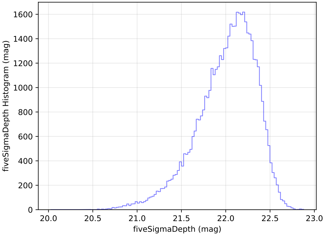
noroll_mjdp60_v3.4_10yrs Yr 1 y band: fiveSigmaDepth Histogram
