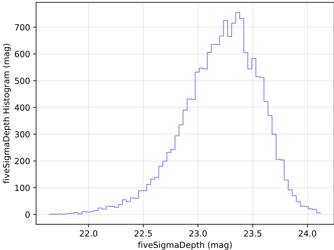
noroll_mjdp60_v3.4_10yrs Yr 1 u band: fiveSigmaDepth Histogram
