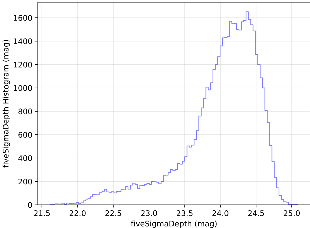
noroll_mjdp60_v3.4_10yrs Yr 1 r band: fiveSigmaDepth Histogram
