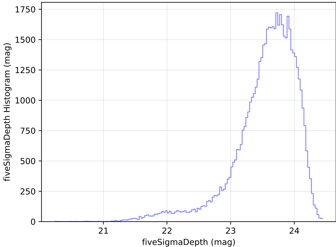
noroll_mjdp60_v3.4_10yrs Yr 1 i band: fiveSigmaDepth Histogram
