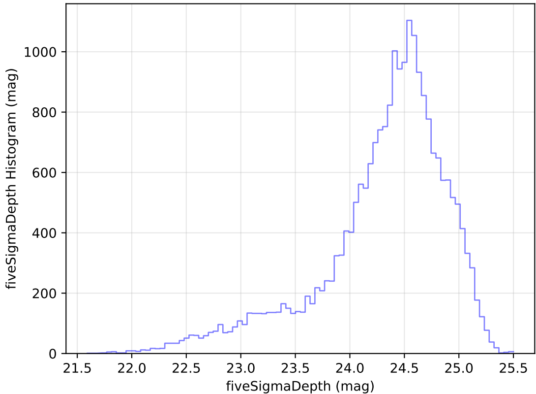
noroll_mjdp60_v3.4_10yrs Yr 1 g band: fiveSigmaDepth Histogram
