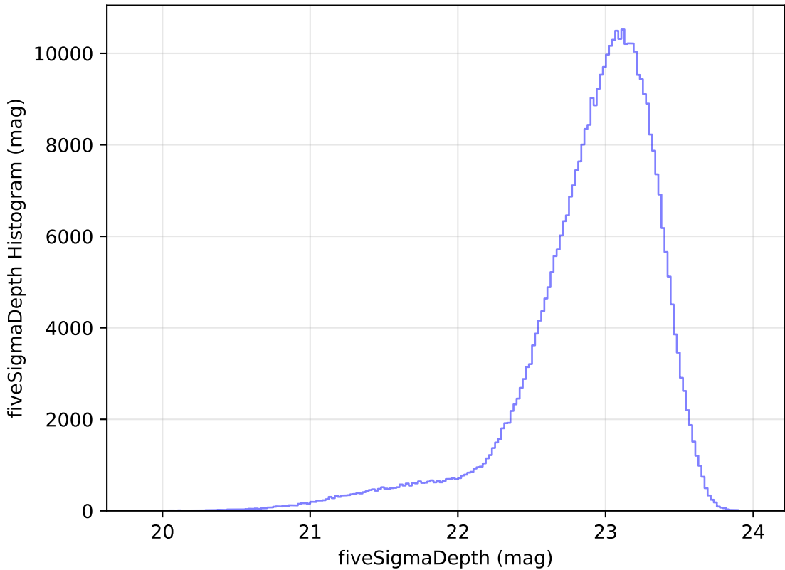
noroll_mjdp60_v3.4_10yrs WFD z band: fiveSigmaDepth Histogram
