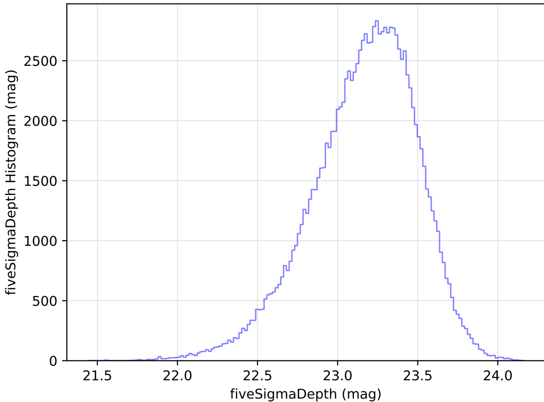
noroll_mjdp60_v3.4_10yrs WFD u band: fiveSigmaDepth Histogram
