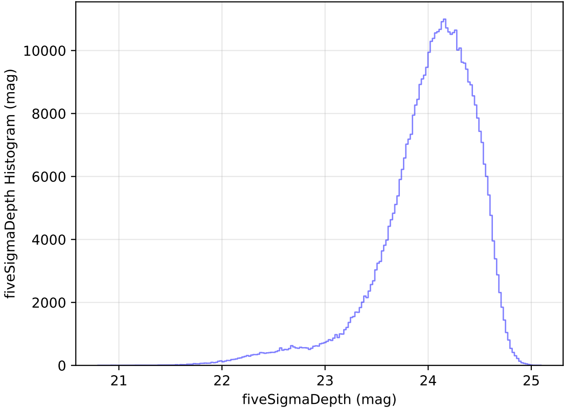
noroll_mjdp60_v3.4_10yrs WFD r band: fiveSigmaDepth Histogram
