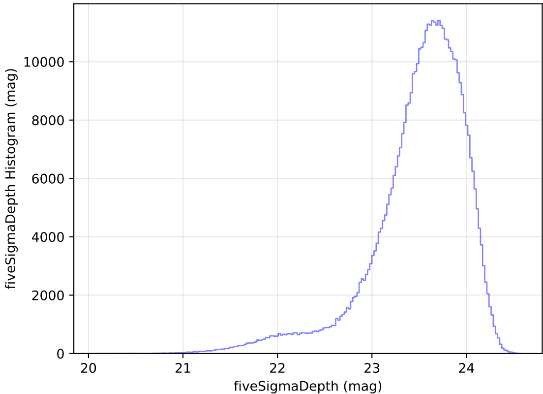
noroll_mjdp60_v3.4_10yrs WFD i band: fiveSigmaDepth Histogram
