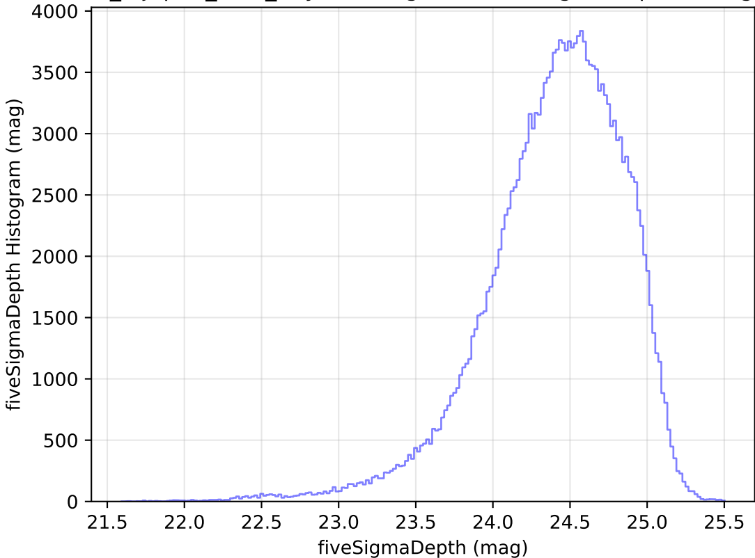
noroll_mjdp60_v3.4_10yrs WFD g band: fiveSigmaDepth Histogram
