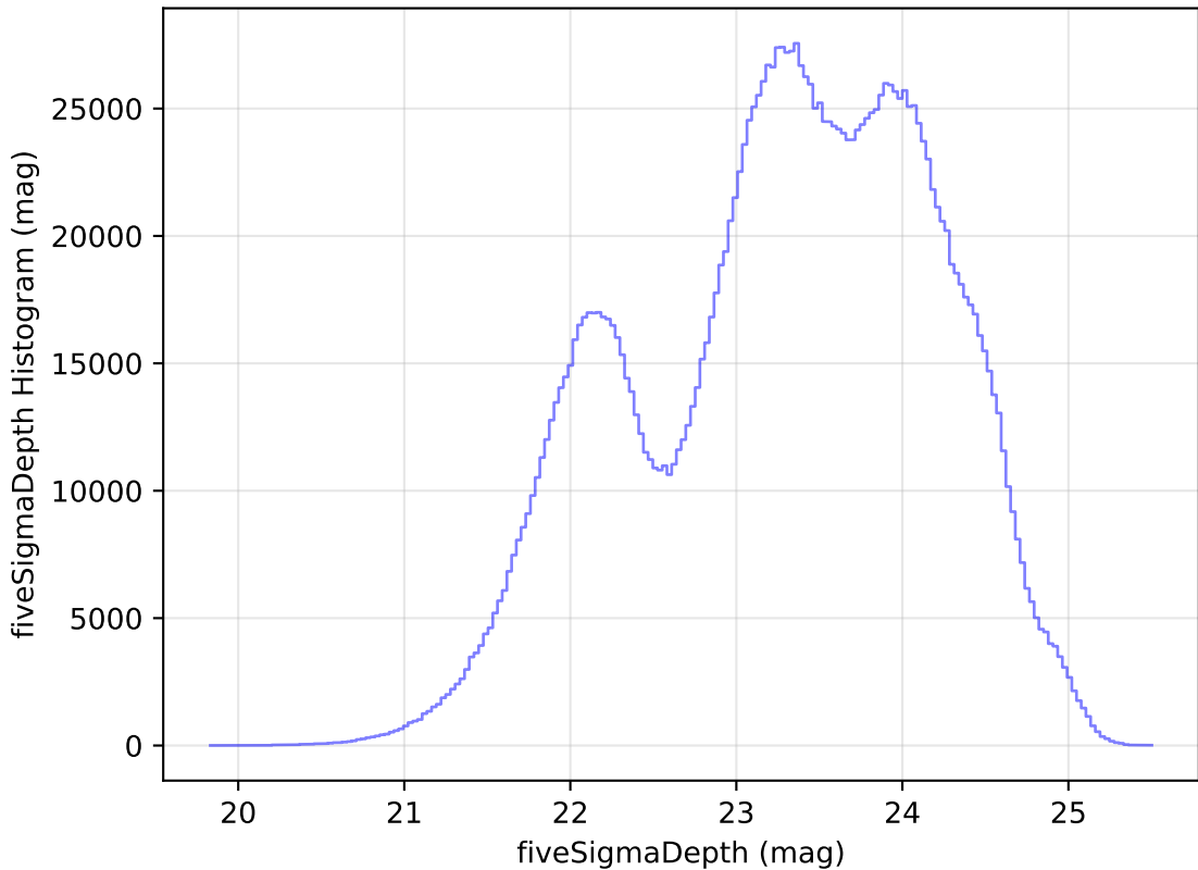
noroll_mjdp60_v3.4_10yrs WFD all bands: fiveSigmaDepth Histogram
