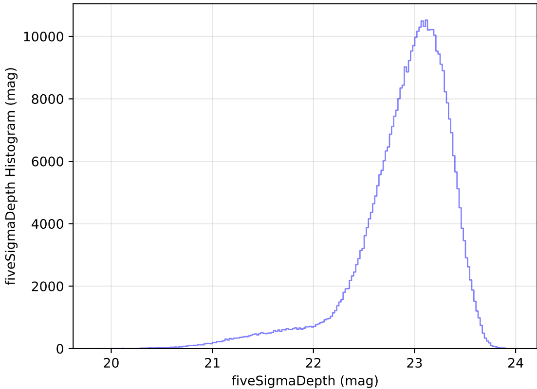
noroll_mjdp60_v3.4_10yrs All sky z band: fiveSigmaDepth Histogram
