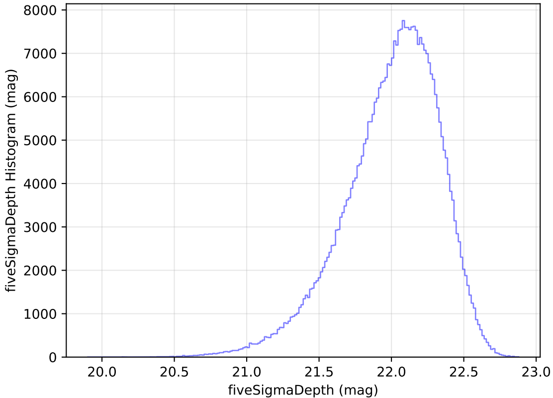
noroll_mjdp60_v3.4_10yrs All sky y band: fiveSigmaDepth Histogram
