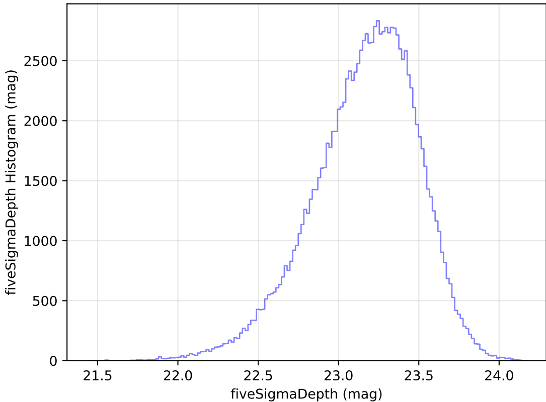
noroll_mjdp60_v3.4_10yrs All sky u band: fiveSigmaDepth Histogram
