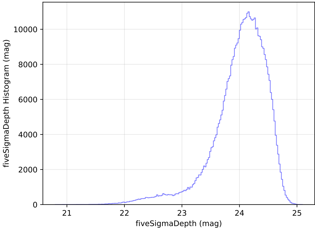
noroll_mjdp60_v3.4_10yrs All sky r band: fiveSigmaDepth Histogram
