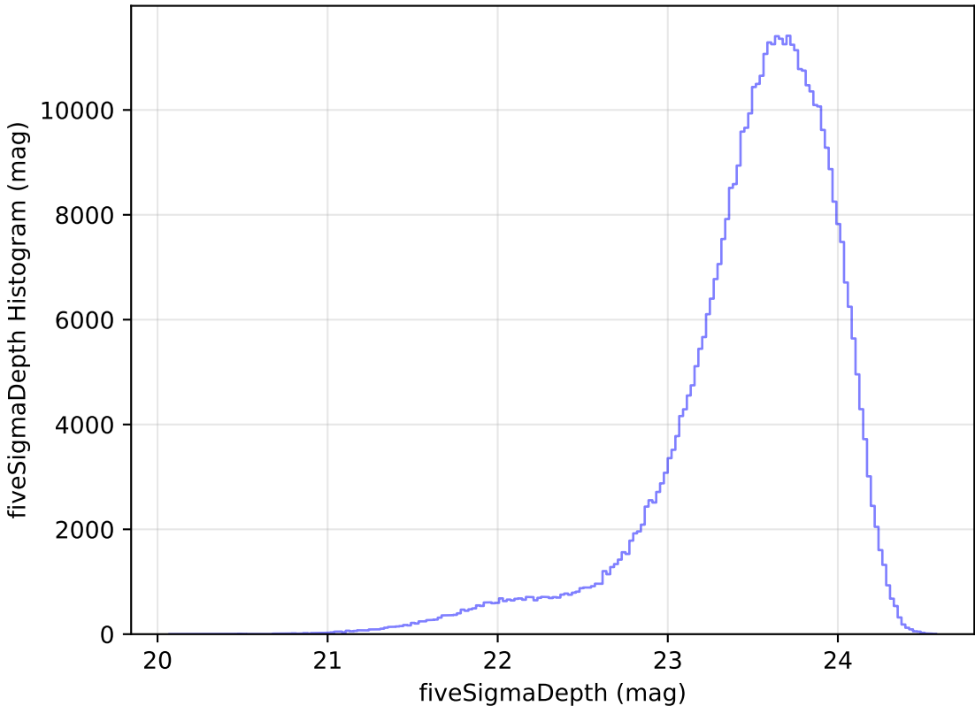
noroll_mjdp60_v3.4_10yrs All sky i band: fiveSigmaDepth Histogram
