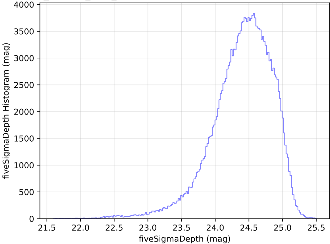
noroll_mjdp60_v3.4_10yrs All sky g band: fiveSigmaDepth Histogram
