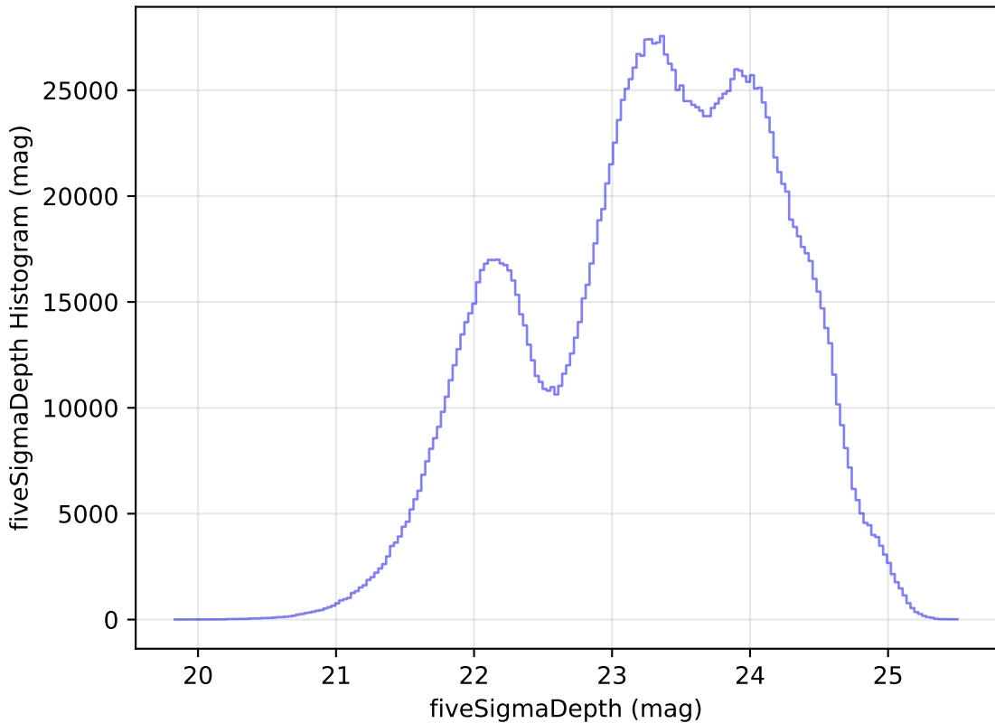
noroll_mjdp60_v3.4_10yrs All sky all bands: fiveSigmaDepth Histogram
