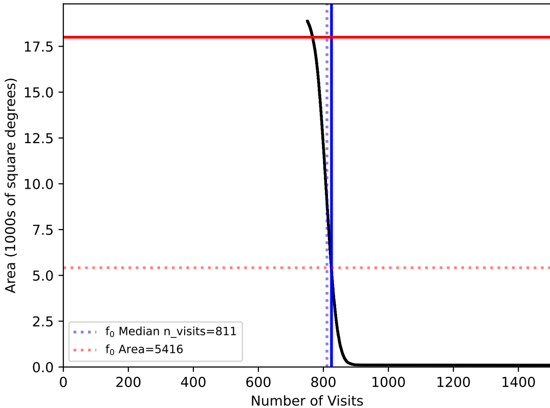
noroll_mjdp60_v3.4_10yrs WFD: fO
