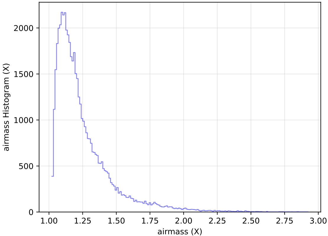
noroll_mjdp60_v3.4_10yrs Yr 1 y band: airmass Histogram
