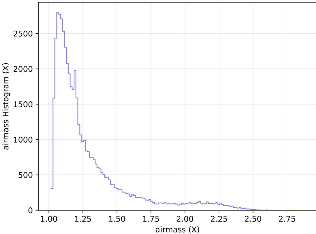
noroll_mjdp60_v3.4_10yrs Yr 1 r band: airmass Histogram
