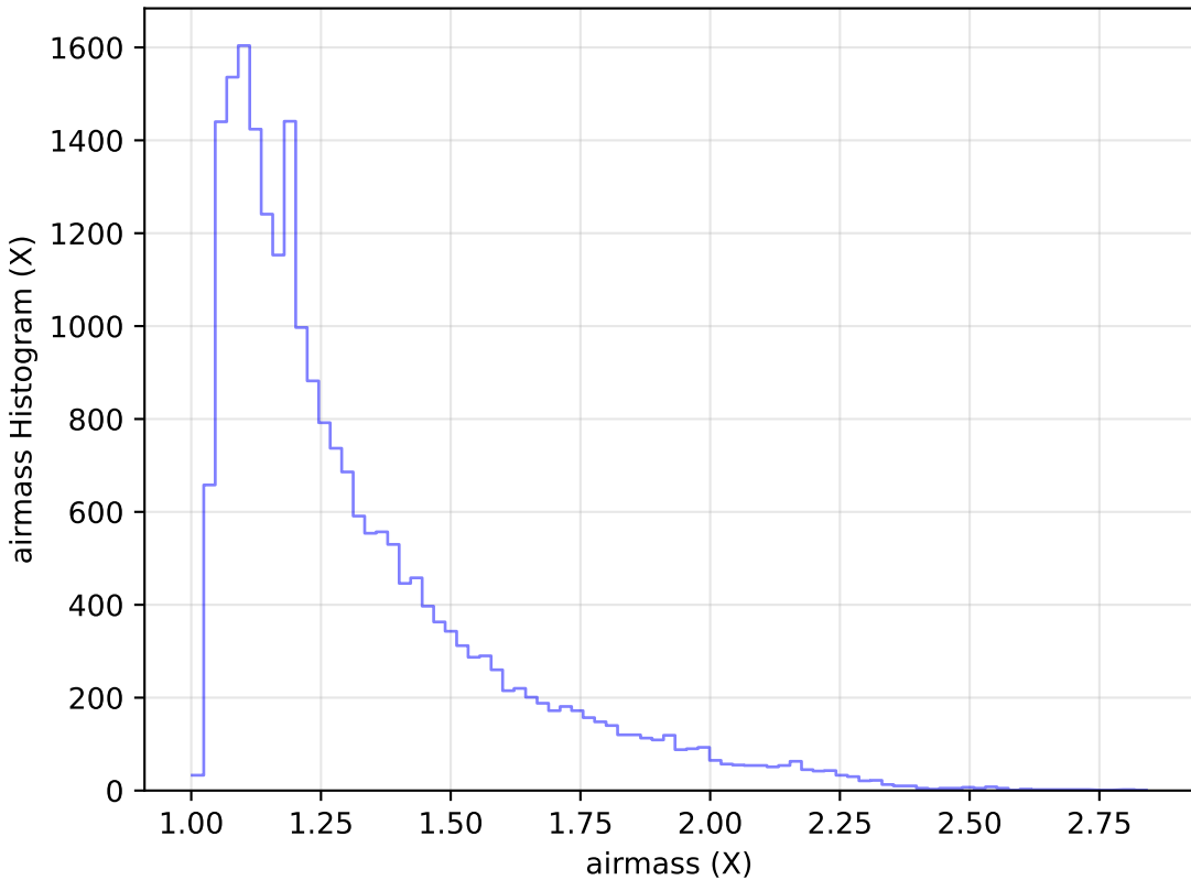
noroll_mjdp60_v3.4_10yrs Yr 1 g band: airmass Histogram
