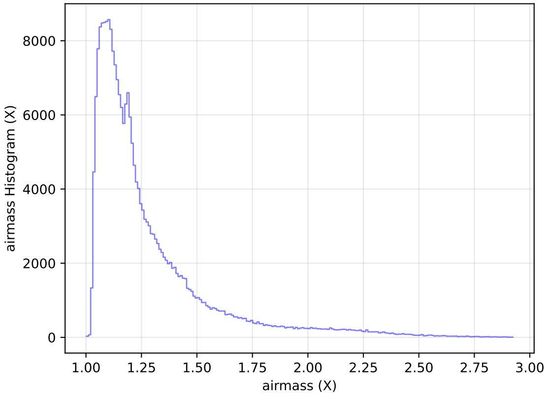
noroll_mjdp60_v3.4_10yrs Yr 1 all bands: airmass Histogram
