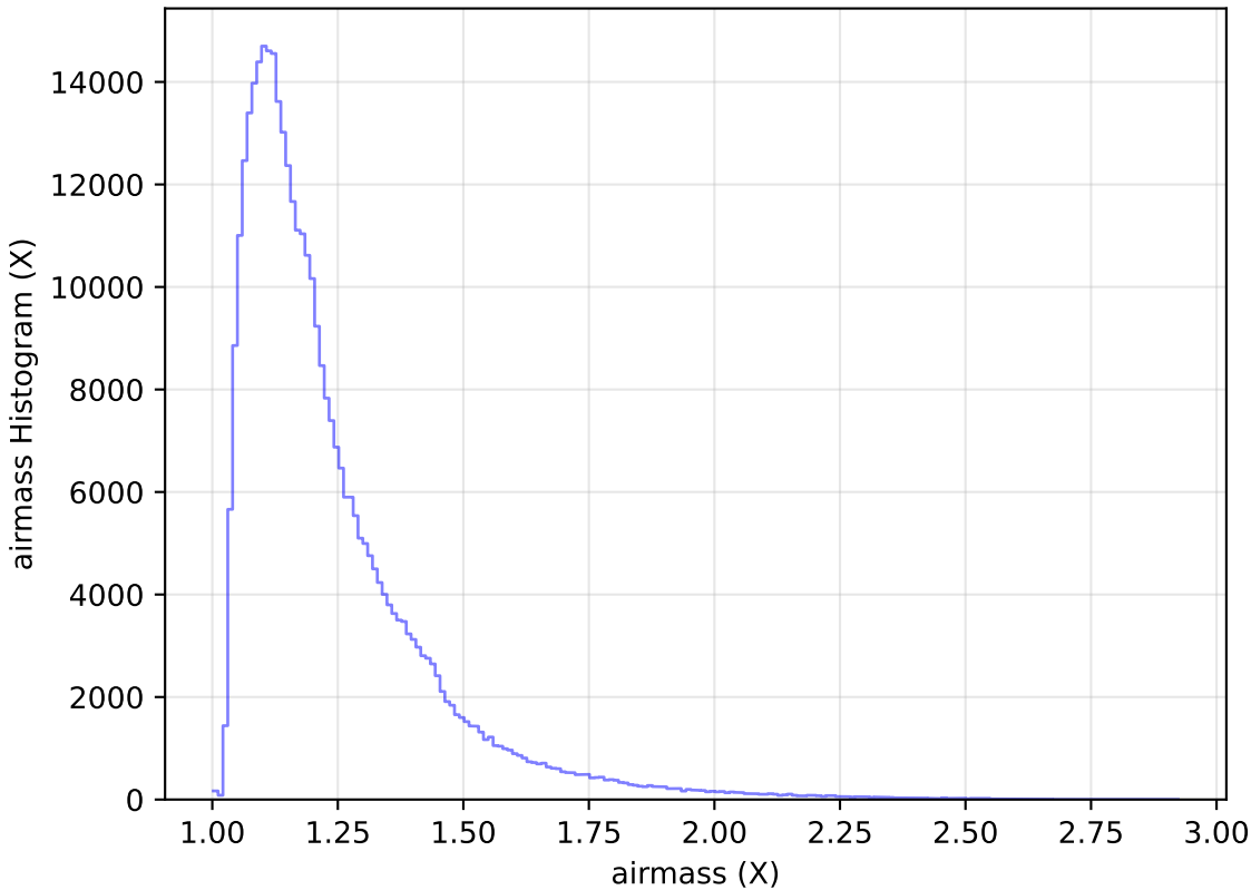
noroll_mjdp60_v3.4_10yrs WFD y band: airmass Histogram
