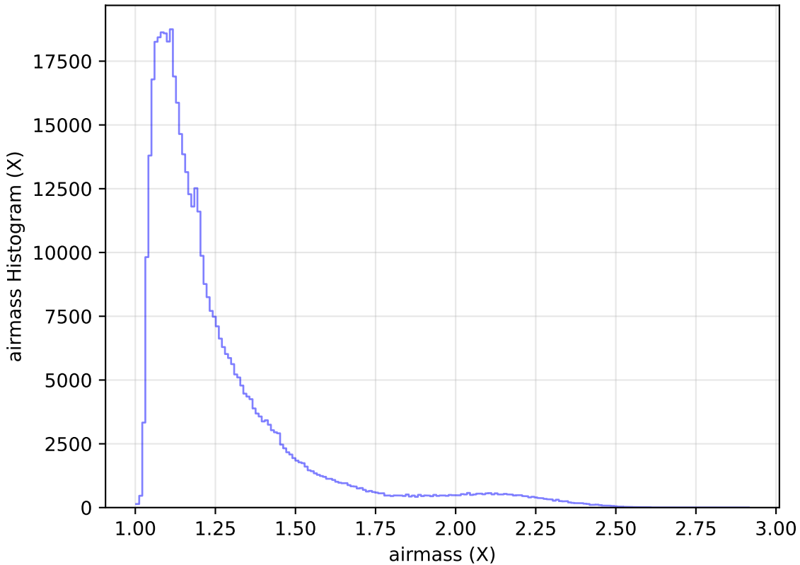
noroll_mjdp60_v3.4_10yrs WFD r band: airmass Histogram
