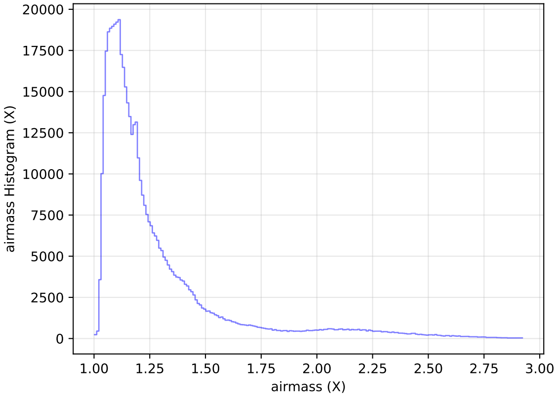
noroll_mjdp60_v3.4_10yrs WFD i band: airmass Histogram
