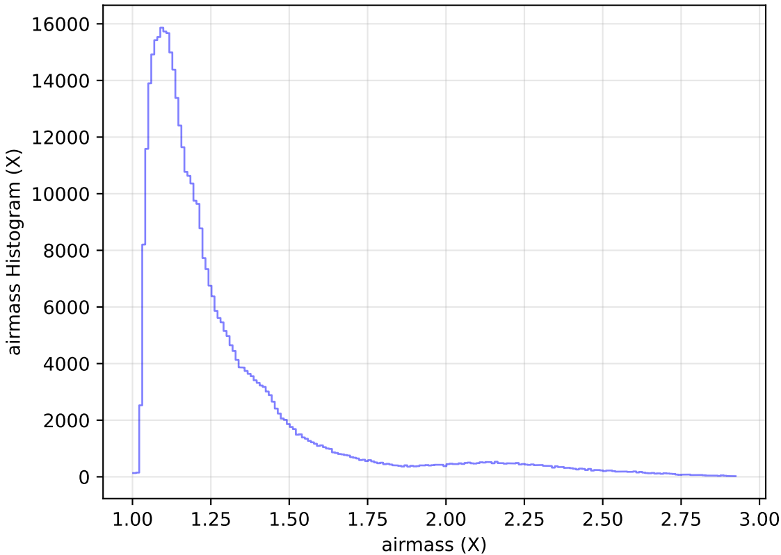
noroll_mjdp60_v3.4_10yrs All sky z band: airmass Histogram
