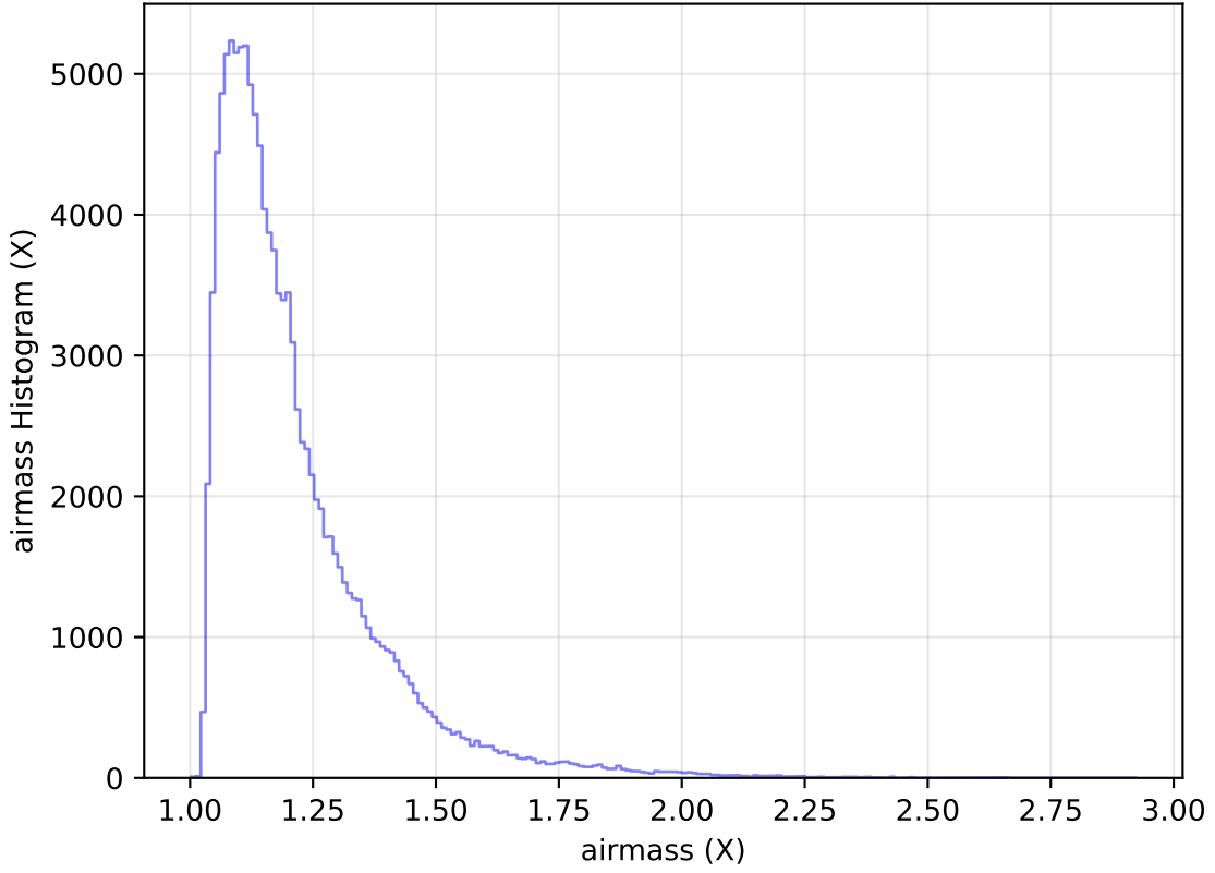
noroll_mjdp60_v3.4_10yrs All sky u band: airmass Histogram
