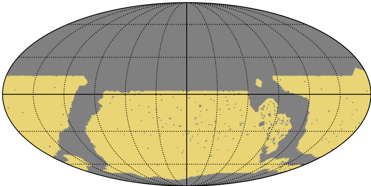
noroll_mjdp60_v3.4_10yrs WFD: RapidRevisits
