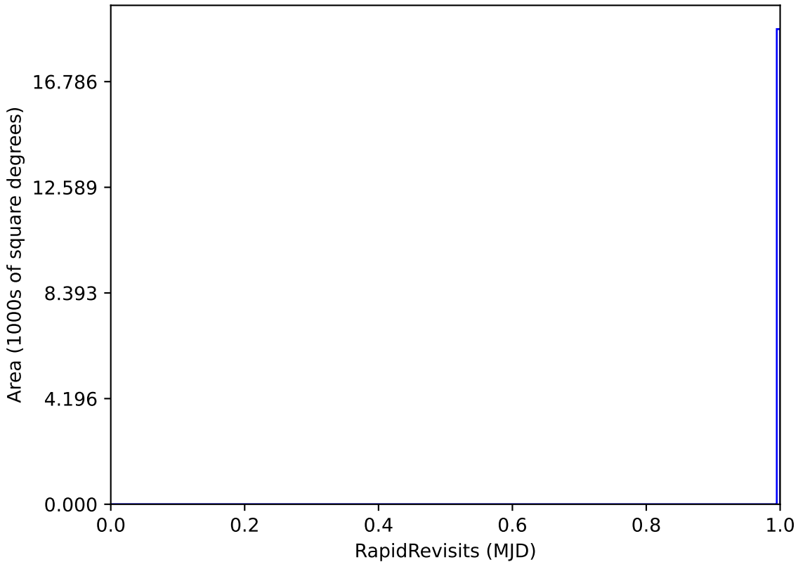
noroll_mjdp60_v3.4_10yrs WFD: RapidRevisits
