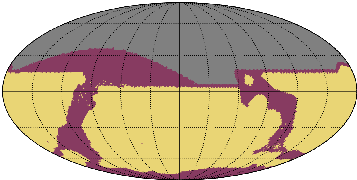
noroll_mjdp60_v3.4_10yrs All sky: RapidRevisits
