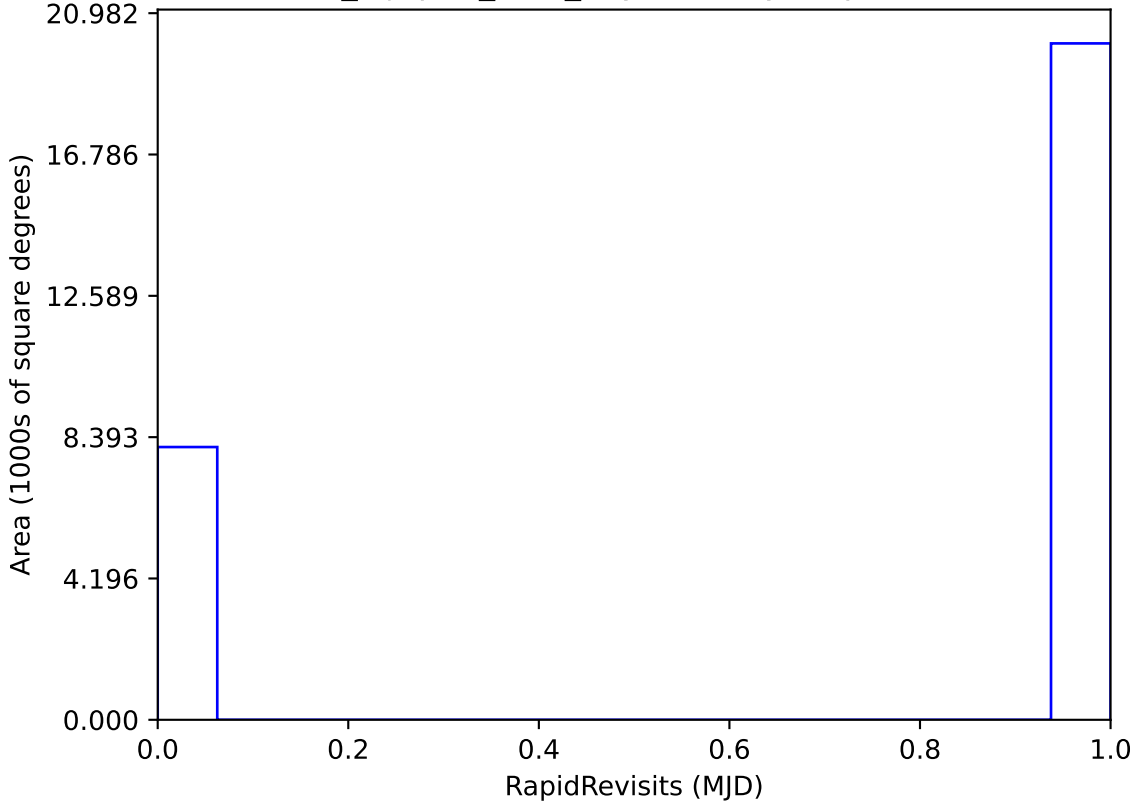
noroll_mjdp60_v3.4_10yrs All sky: RapidRevisits
