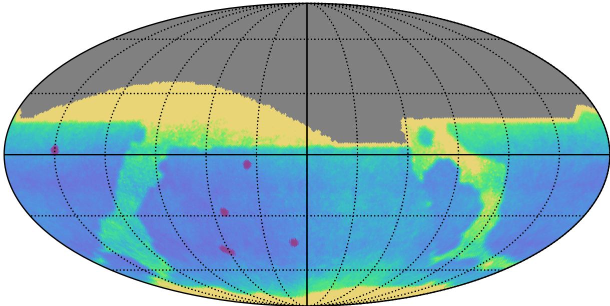
noroll_mjdp60_v3.4_10yrs All sky: Proper Motion Uncert @ 24.0
