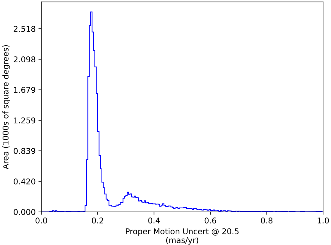
noroll_mjdp60_v3.4_10yrs All sky: Proper Motion Uncert @ 20.5
