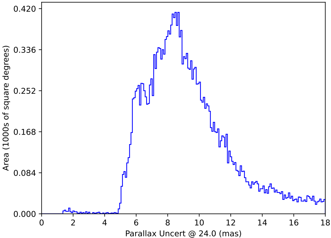
noroll_mjdp60_v3.4_10yrs All sky: Parallax Uncert @ 24.0
