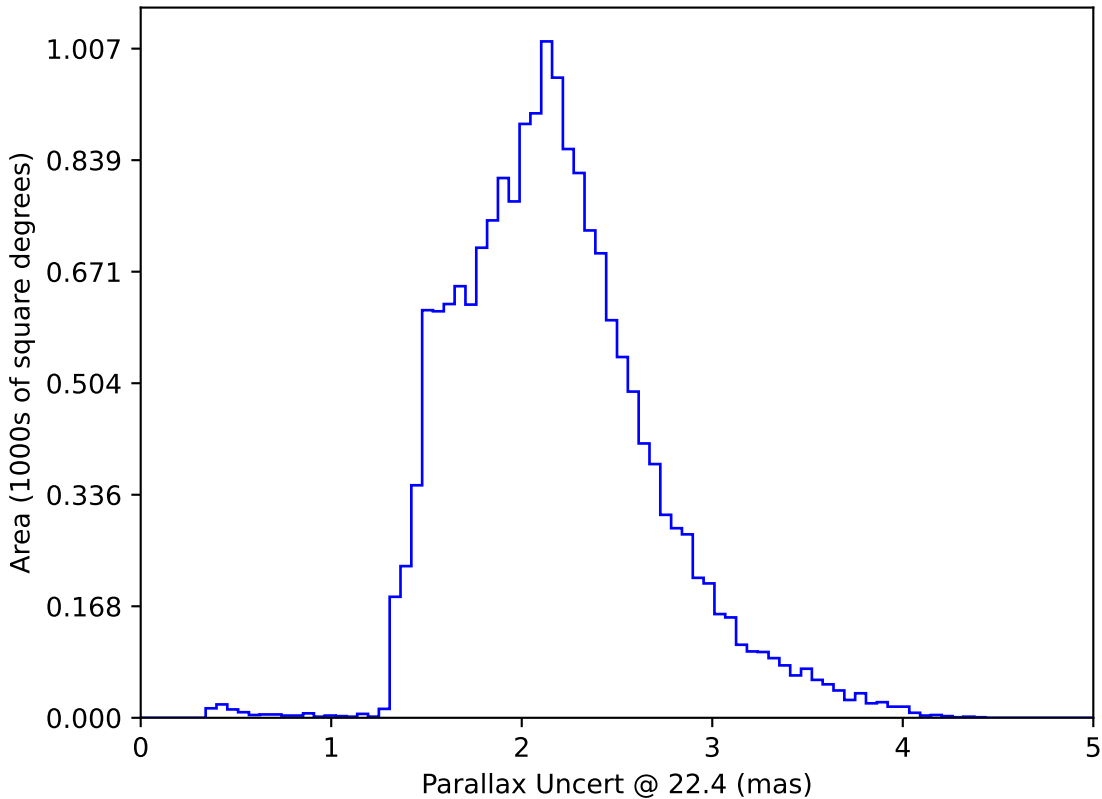
noroll_mjdp60_v3.4_10yrs WFD: Parallax Uncert @ 22.4
